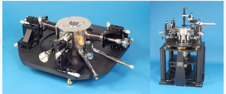
Probe station
