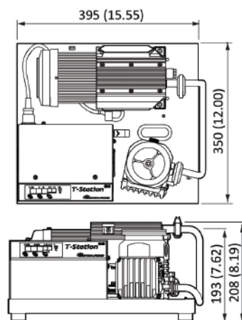
T-Station 85H Dry with XDD1 backing pump
